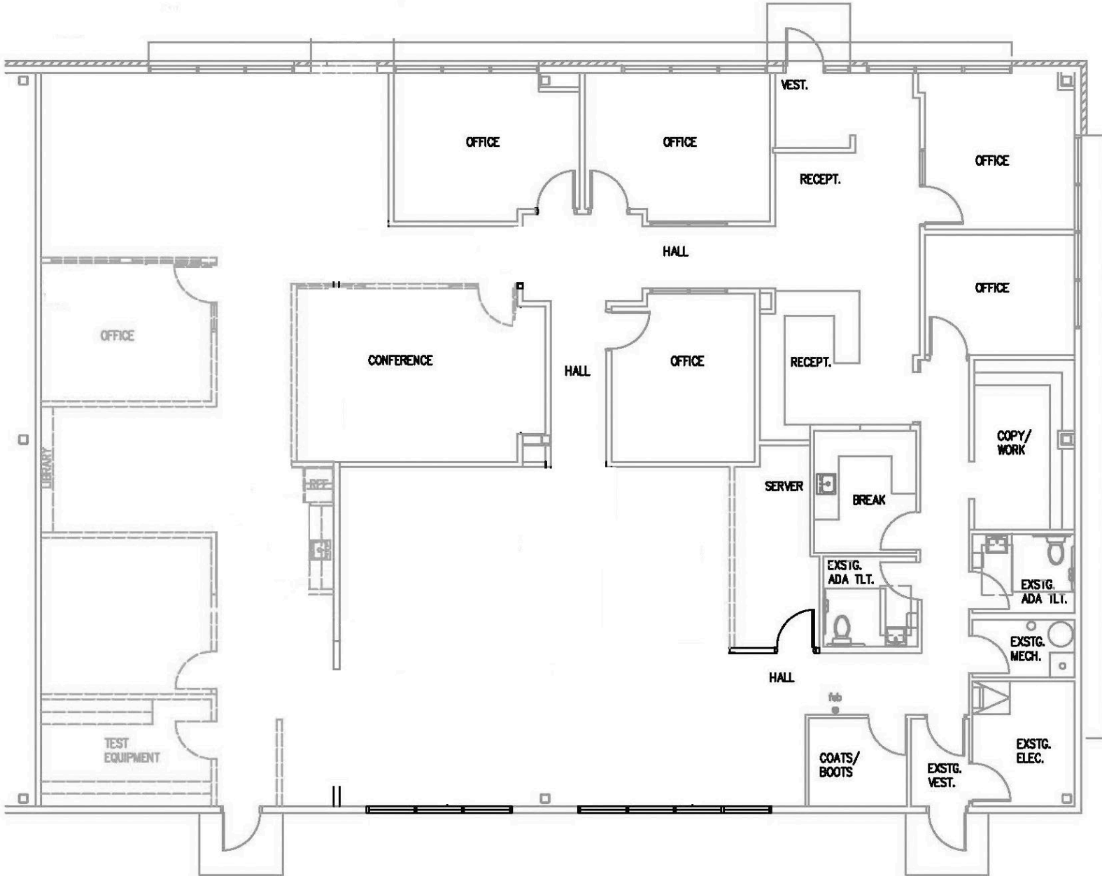
FLOOR PLAN 1/8"=1'-0"
